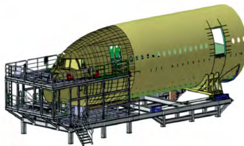
Tooling and assembly lines from welded aluminium or steel frameworks
